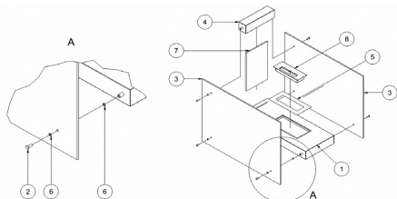
Picture 4. Mounting of biofireplace – Linate
