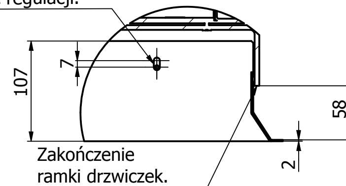
C (1:4)
