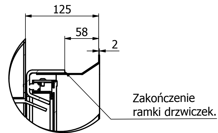
A (1:4)
