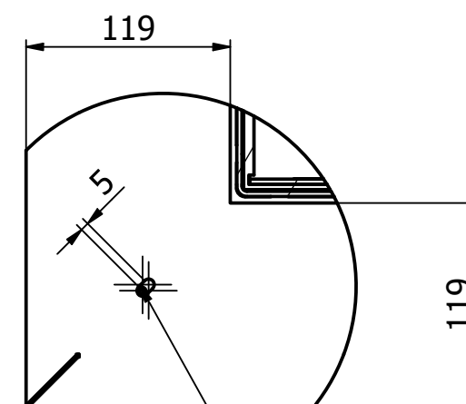
E (1:4)
