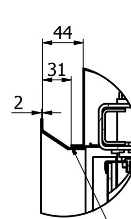
A (1:4)
