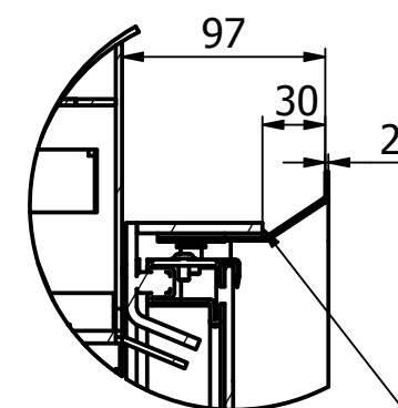
C (1:4)
