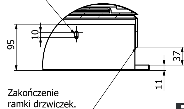
C (1:4)
