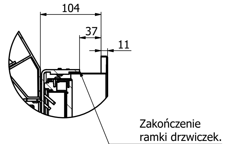
A (1:4)
