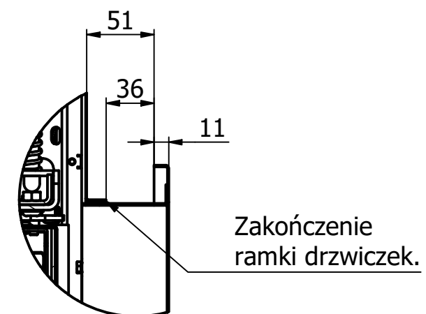
A (1:4)
