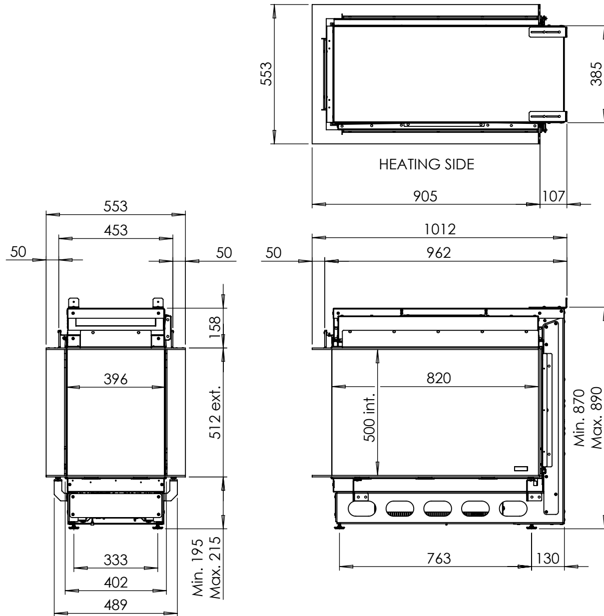
Dimensional Drawing e-MatriX Mood 800/500 RD
