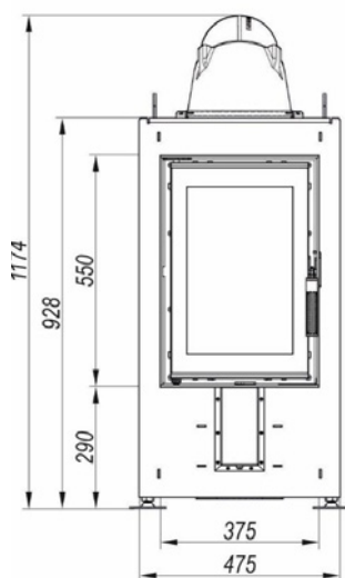
Vis XSM 6C
